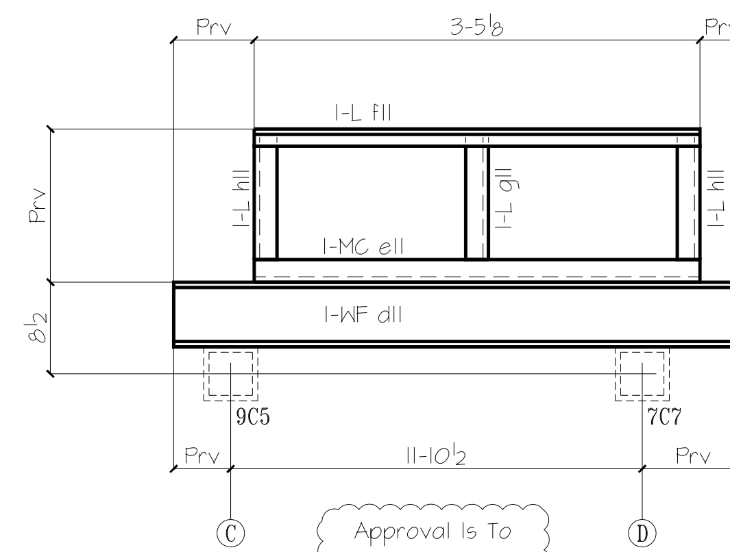
3 Sun Canopy MK: 11SC1 Ref 7/53.1
