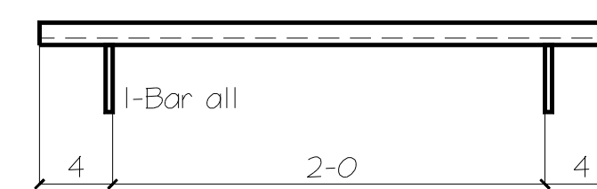
1 Shades Brackets MK: 11SB7 Per Sun Shades 11SS9
