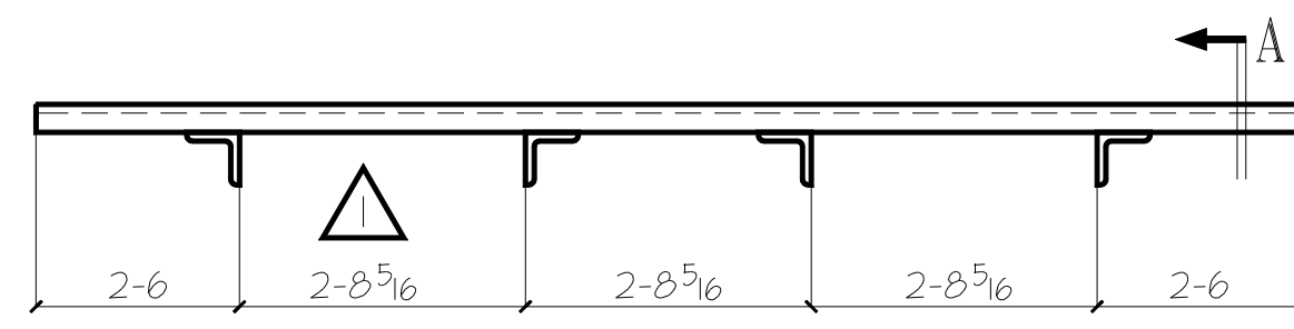
1 Sun Shades MK: 11SS6 9/53.1 A2.0 Per Window Type T
