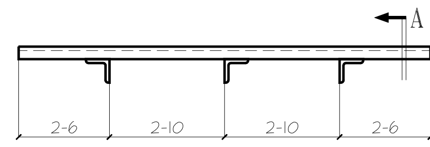
3 Sun Shades MK: 11SS5 9/53.1 A2.0 Per Window Type U
