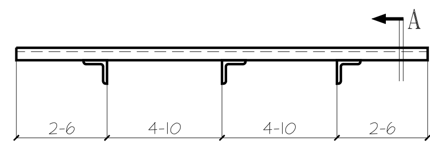
1 Sun Shades MK: 11SS10 9/53.1 A2.0 Per Window Type M
