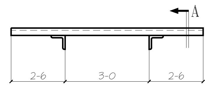
7 Sun Shades MK: 11SS1 9/53.1 A2.0 Per Window Type R
