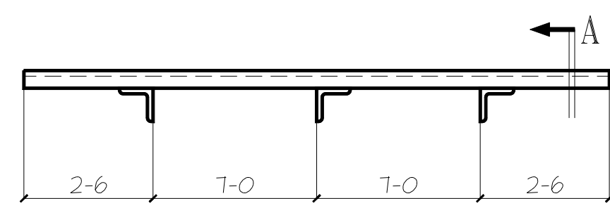
1 Sun Shades MK: 11SS3 9/53.1 A2.0 Per Window Type P
