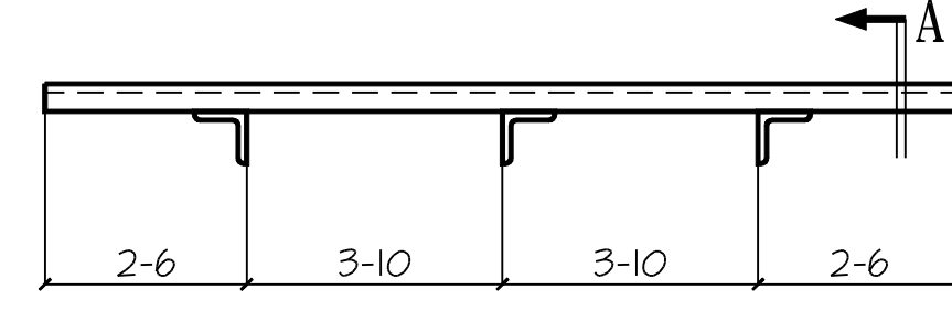
2 Sun Shades MK: 11SS8 9/53.1 A2.0 Per Window Type I
