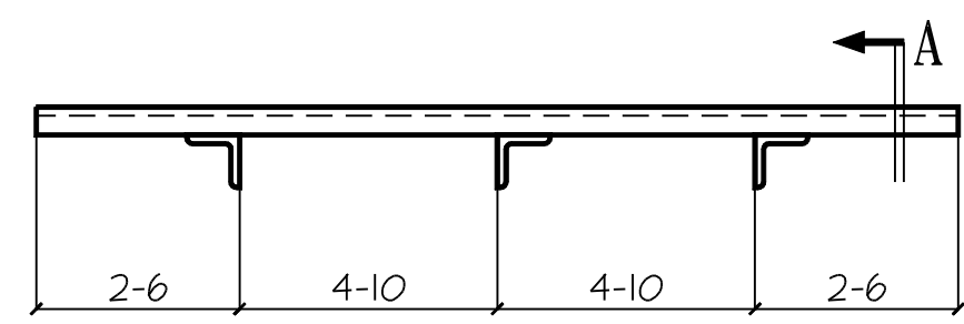
1 Sun Shades MK: 11SS10 9/53.1 A2.0 Per Window Type M
