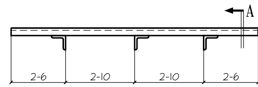
3 Sun Shades MK: 11SS5 9/53.1 A2.0 Per Window Type U
