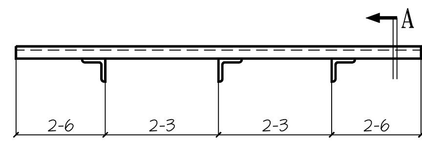
2 Sun Shades MK: 11SS2 9/53.1 A2.0 Per Window Type H
