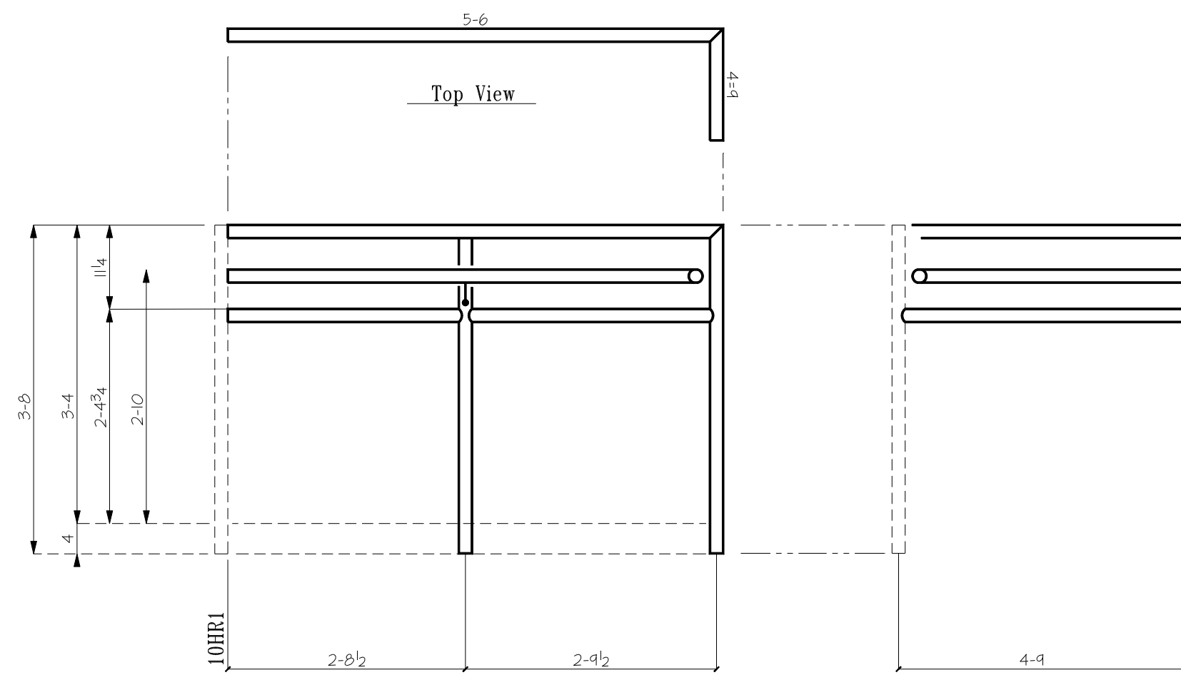
1 Handrails Mk 51HR2 Fabricate As Shown
