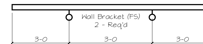
1 Wallrails Mk 50WR6 Fabricate As Shown
