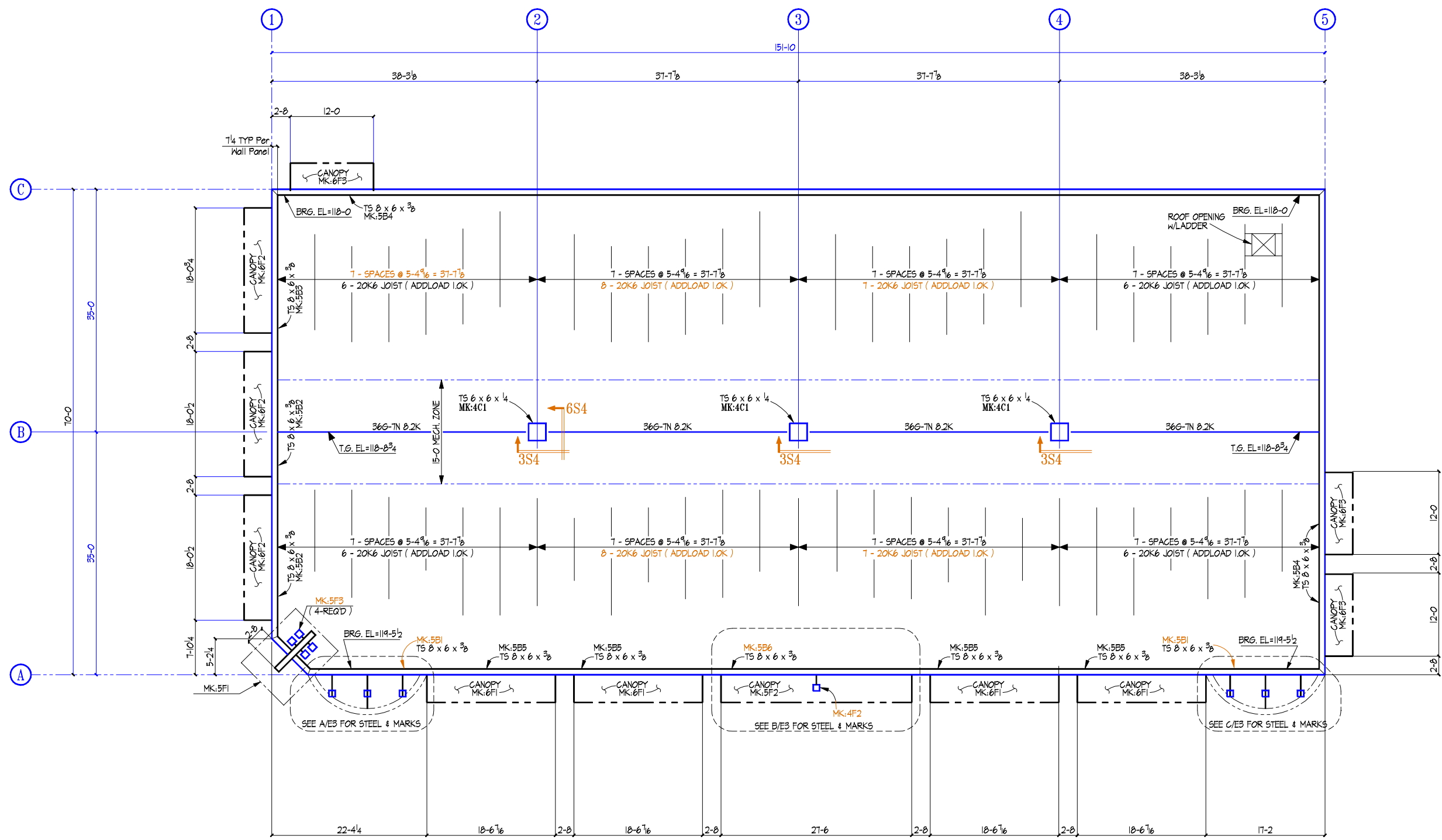
FRAMING PLAN PLAN NORTH → N
